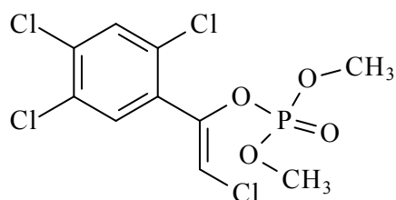
(1 Z )-2-chloro-1-(2,4,5-trichlorophenyl)ethenyl dimethyl phosphate (CAS No., 22248-79-9)
